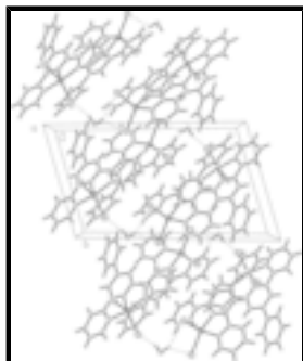
Fig. 2. A view of the crystal packing along the a axis, showing the hydrogen bonding scheme. Hydrogen bonds are represented by dashed lines.
